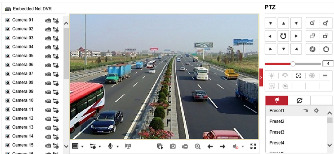
Figure 9-2 Live View
