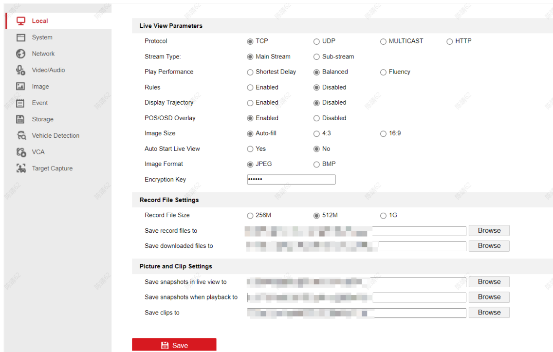
Figure 9-4 Configuration
