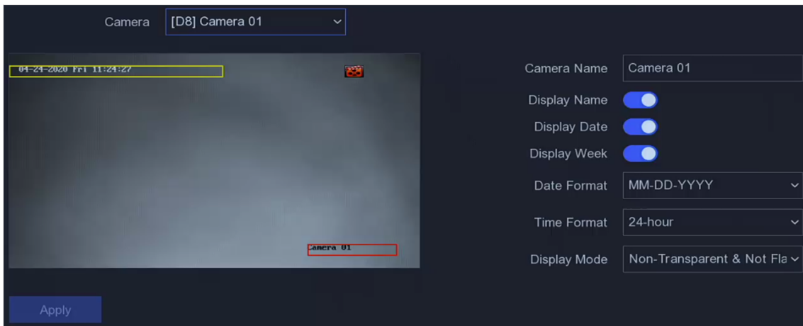
Figure 5-8 OSD
