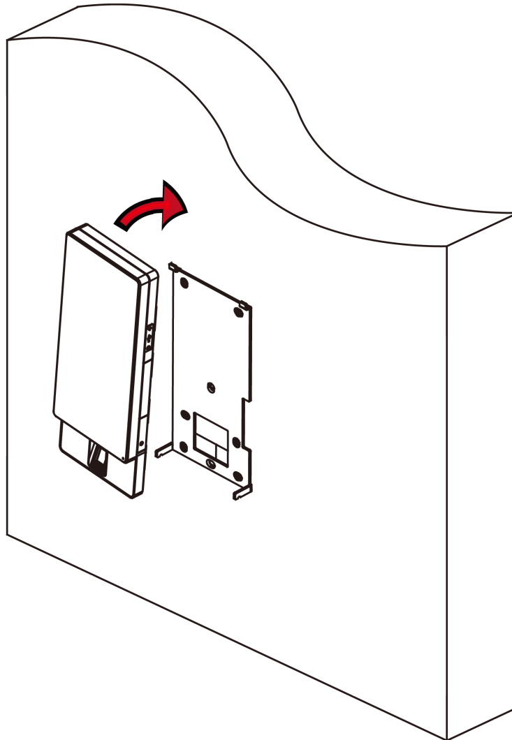
Figure 3-5 Install Device
