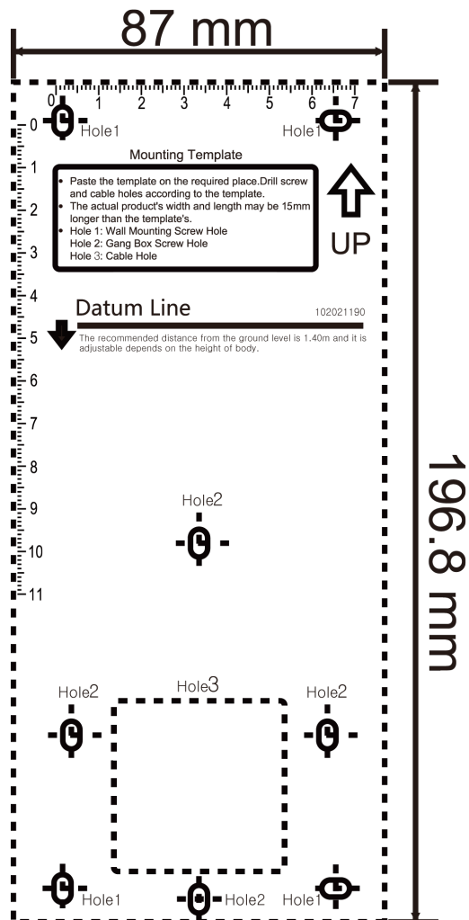
Figure 3-7 Mounting Template
