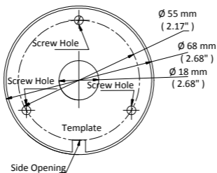
Figure 2-8 Drill Template
