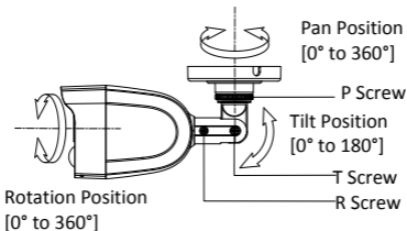
Figure 2-3 3-axis Adjustment
