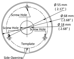
Figure 2-1 Drill Template
