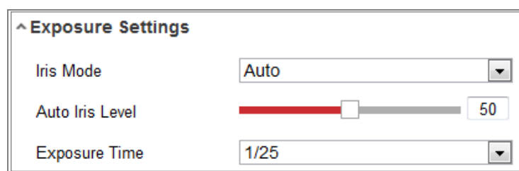
Figure 7-2 Exposure Settings
