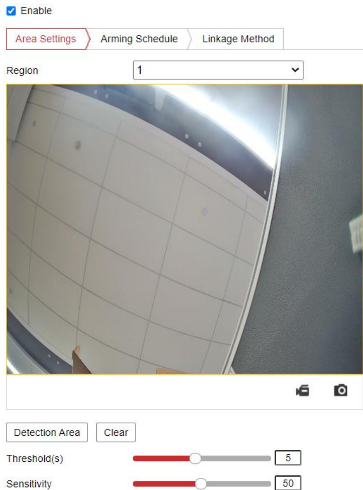
Figure 8-17 Loitering Detection
