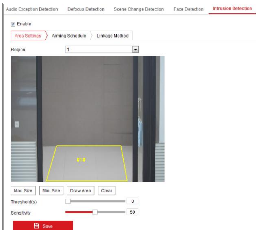
Figure 8-11 Intrusion Detection
