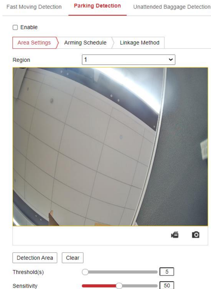
Figure 8-20 Parking Detection
