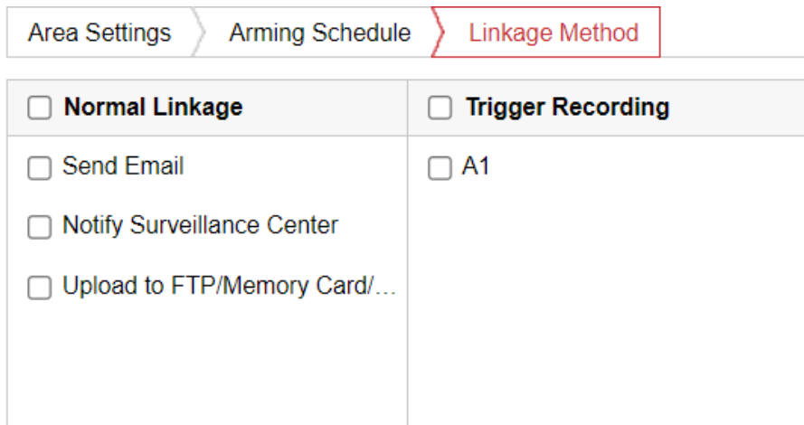
Figure 8-4 Linkage Method
