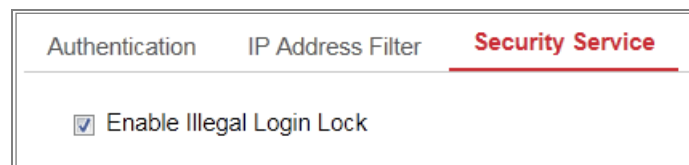
Figure 4-11 Security Service
