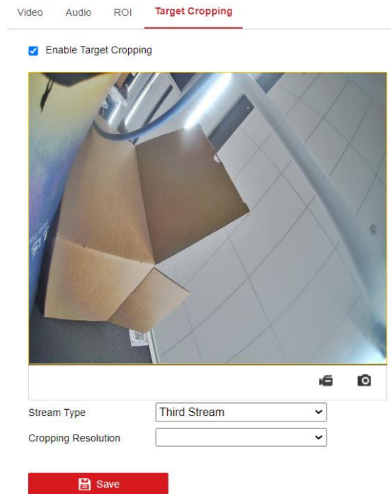
Figure 6-4 Target Cropping
