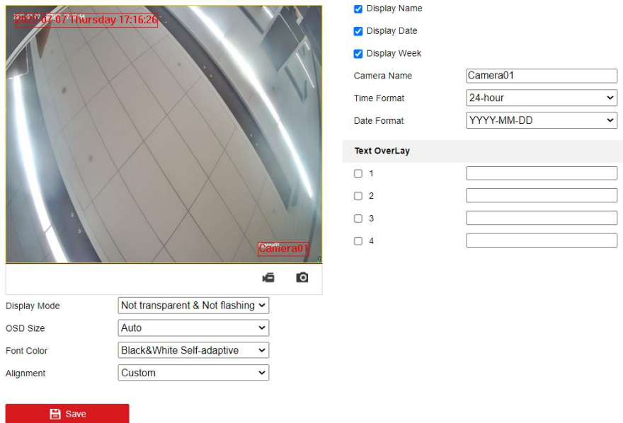
Figure 7-6 OSD Settings
