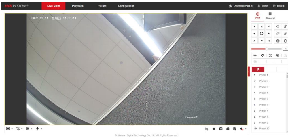
Figure 2-7 Main Interface
