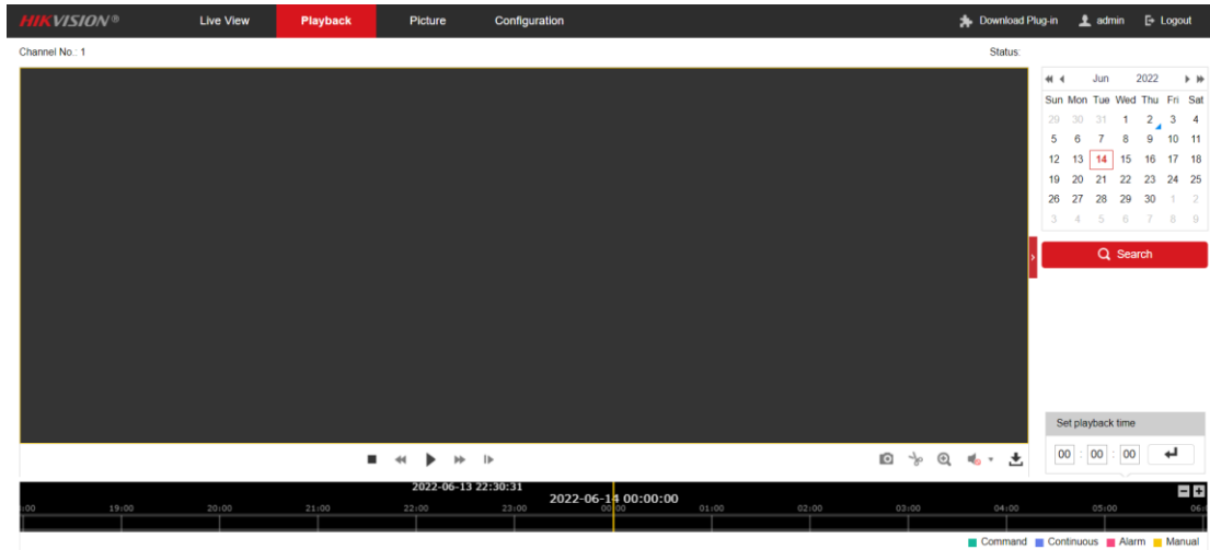
Figure 3-4 Playback Interface
