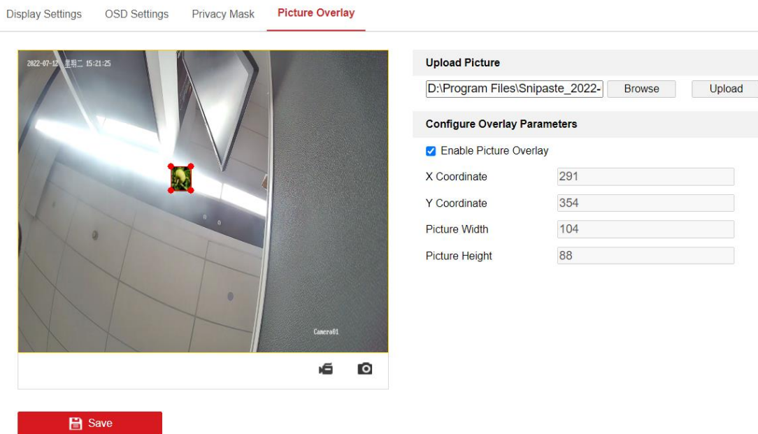
Figure 7-8 Picture Overlay
