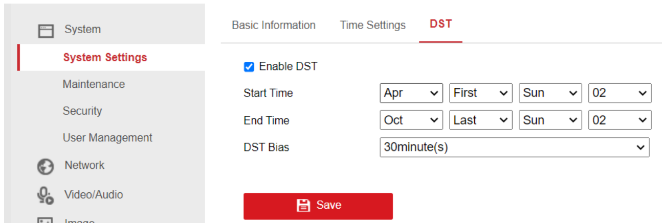
Figure 4-4 DST Settings
