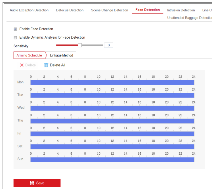
Figure 8-10 Face Detection
