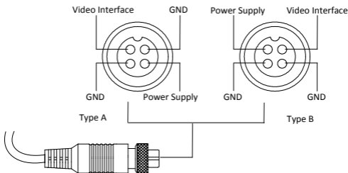
Figure 1-2 Interfaces of Aviation Plug
