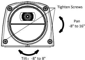
Figure 2-7 Tighten Screws and Adjust Camera
