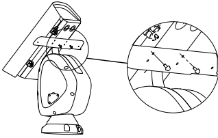
Figure 2-2 Fixation du support infrarouge
