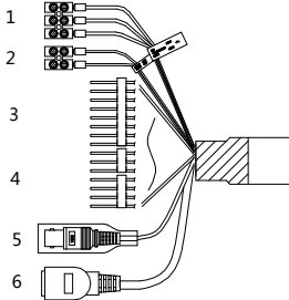
Figure 1-4 : câbles I
