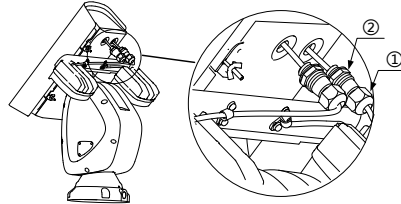
Figure 2-5 Route the Cables 5. Connect the cables of IR modules.
