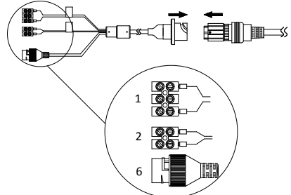
Figure 1-5 Cables II
