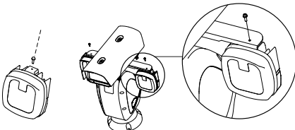
Figure 2-3 Secure the IR Module 3. Secure the buckles to IR bracket with two
