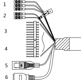
Figure 1-4 Cables I
