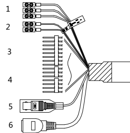
Figur 1-4 Kabler I
