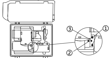
Figure 2-11 Adjust the Laser (Type III of DY9 Series)
