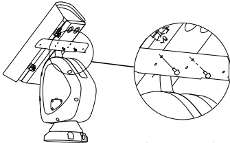
Figure 2-2 Secure the IR Bracket 2. Secure the IR module to the IR bracket with screws.
