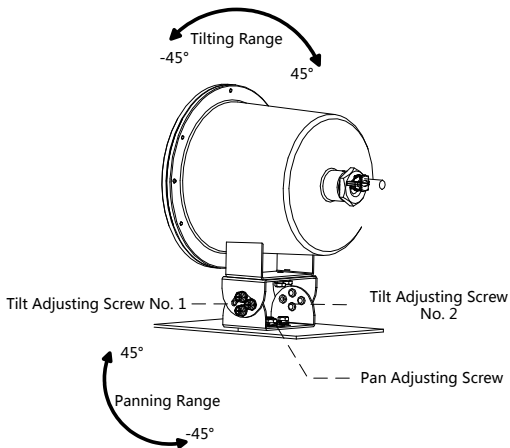
Figure 2-6 2-Axis Adjustment
