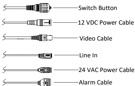
Figure 1-1 Cable Description
