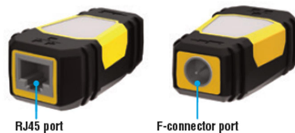
RJ45 port
